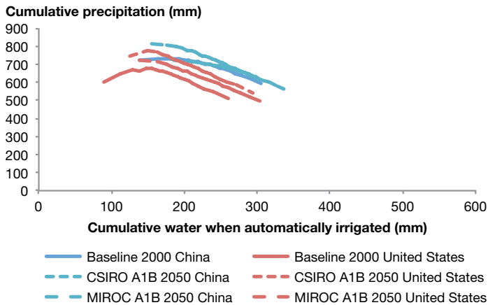
FIGURE A.8 Growing season precipitation by drought intensity compared to the baseline scenario, winter wheat, China and the United States
