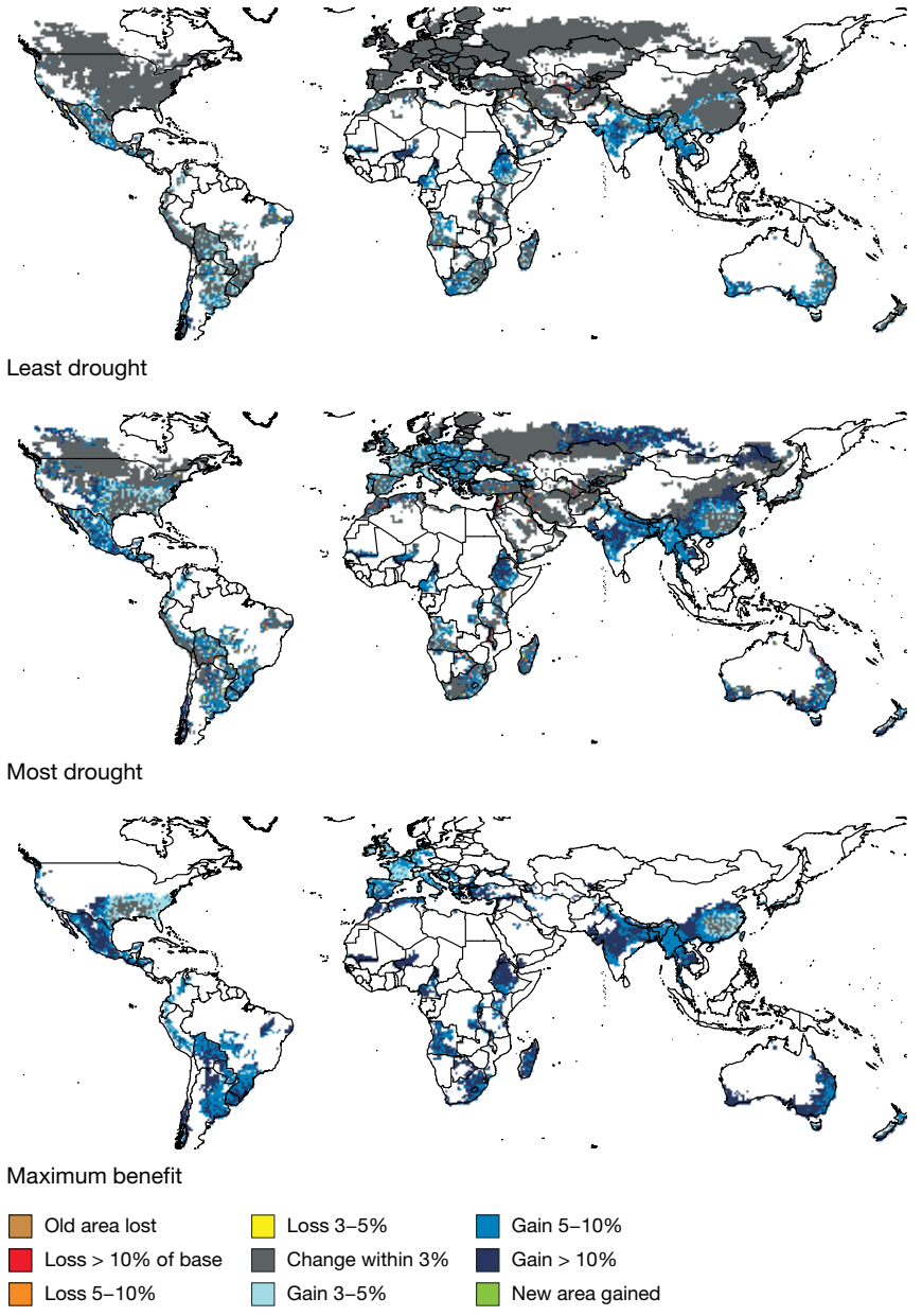
FIGURE A.4A Drought impact maps for winter wheat, baseline scenario, 2000
