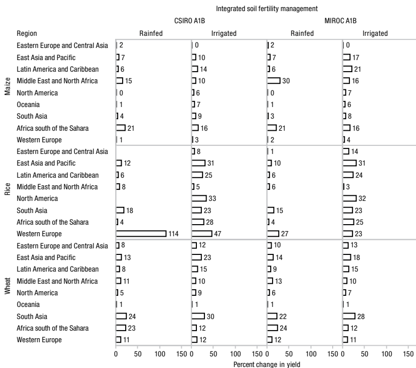
FIGURE 4.8 Regional yield impacts compared to the baseline scenario, by crop and cropping system, integrated soil fertility management, MIROC A1B and CSIRO A1B scenarios, 2050 (%)
