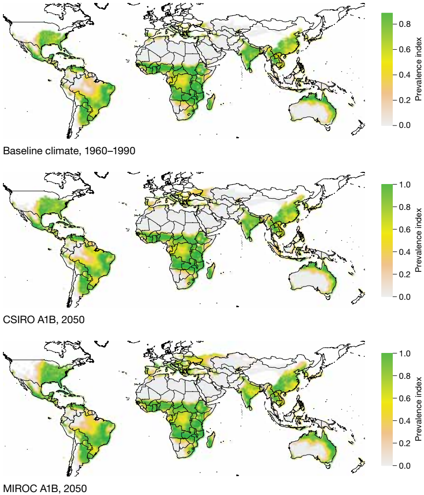
FIGURE C.8 Prevalence of rice weed (barnyardgrass) under baseline climate, CSIRO A1B, and MIROC A1B scenarios
