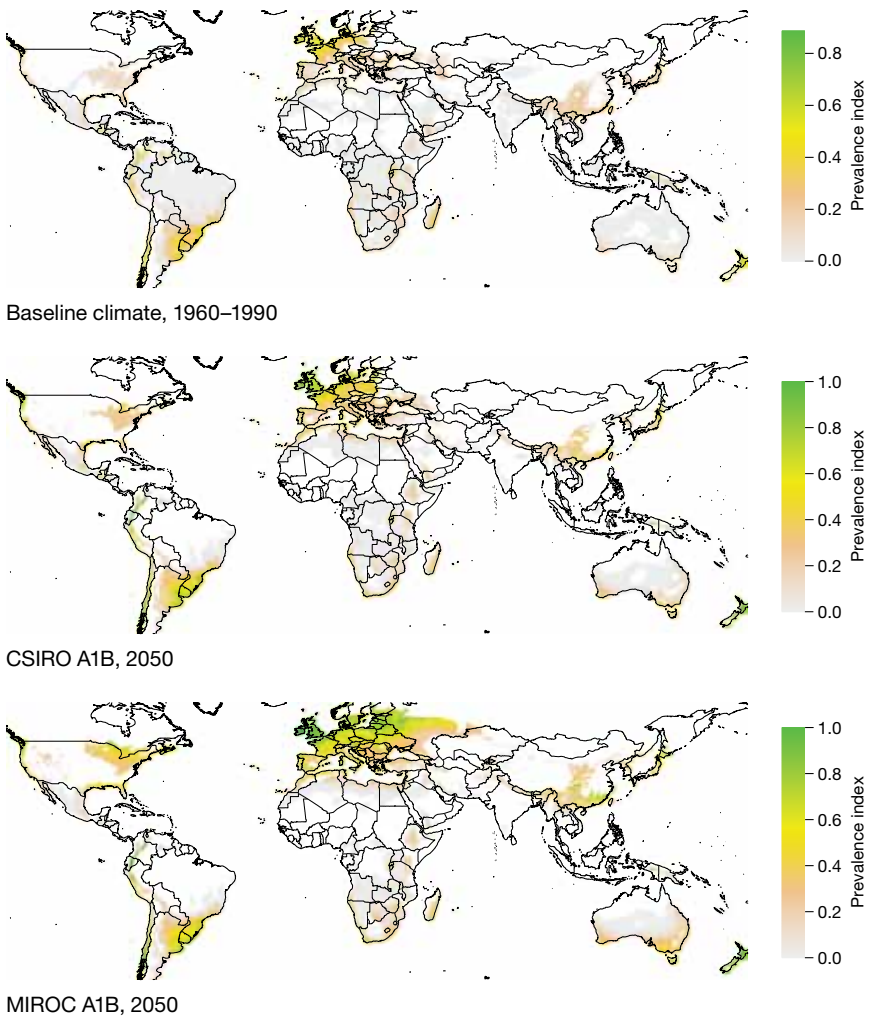
FIGURE C.9 Prevalence of wheat disease (stripe rust) under baseline climate, CSIRO A1B, and MIROC A1B scenarios
