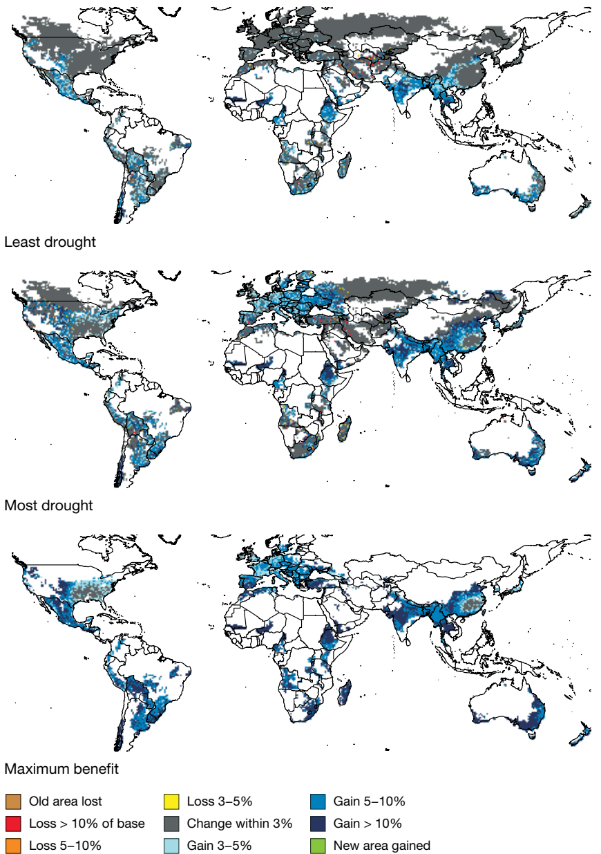
FIGURE A.4C Drought impact maps for winter wheat, MIROC A1B scenario, 2050
