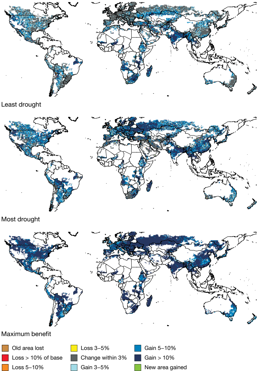
FIGURE A.3C Drought impact maps for spring wheat, MIROC A1B scenario, 2050
