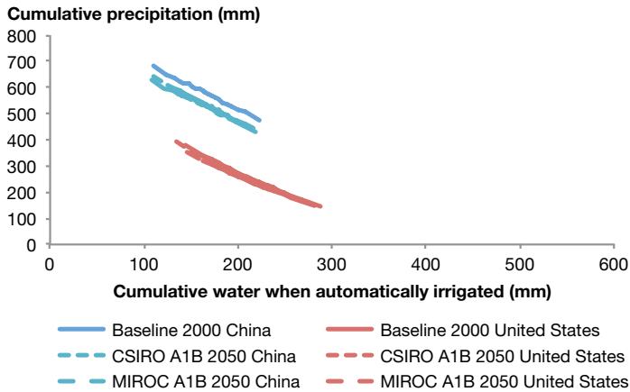
FIGURE A.7 Growing season precipitation by drought intensity compared to the baseline scenario, spring wheat, China and the United States
