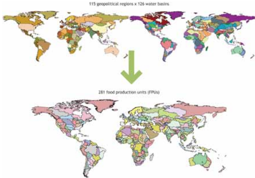
FIGURE A.2 IMPACT model units of analysis, the food-producing unit
