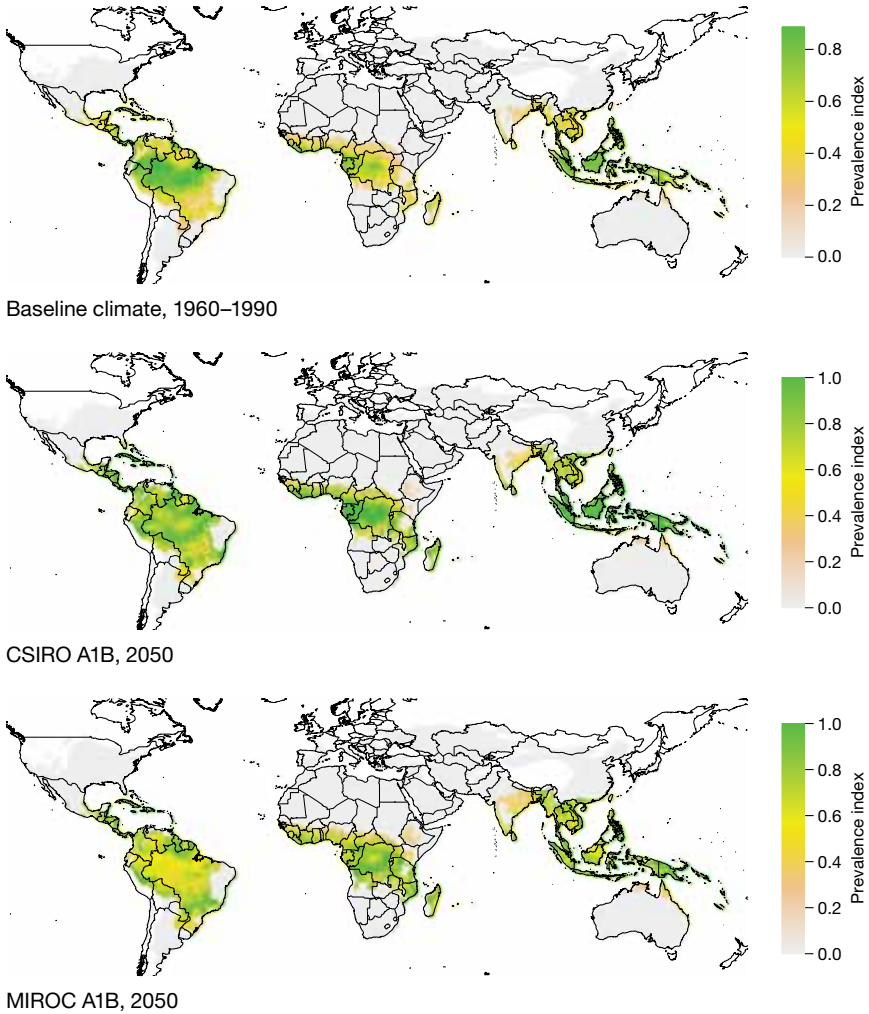
FIGURE C.12 Prevalence of rice pest (yellow stem borer) under baseline climate, CSIRO A1B, and MIROC A1B scenarios
