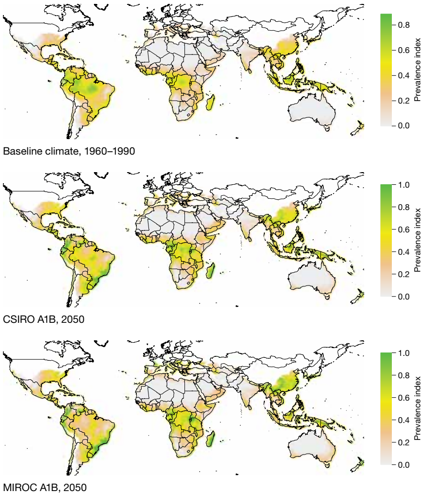
FIGURE C.2 Prevalence of maize disease (common rust) under baseline climate, CSIRO A1B, and MIROC A1B scenarios
