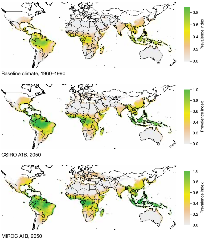
FIGURE C.1 Prevalence of maize disease (grey leaf spot) under baseline climate, CSIRO A1B, and MIROC A1B scenarios
