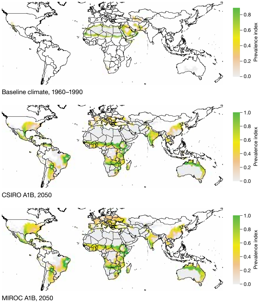
FIGURE C.4 Prevalence of maize weed (Johnson grass) under baseline climate, CSIRO A1B, and MIROC A1B scenarios
