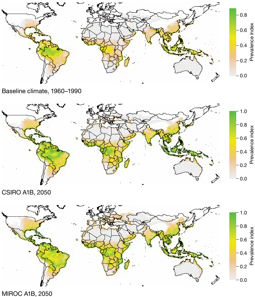
FIGURE C.6 Prevalence of rice pest (striped stem borer) under baseline climate, CSIRO A1B, and MIROC A1B scenarios
