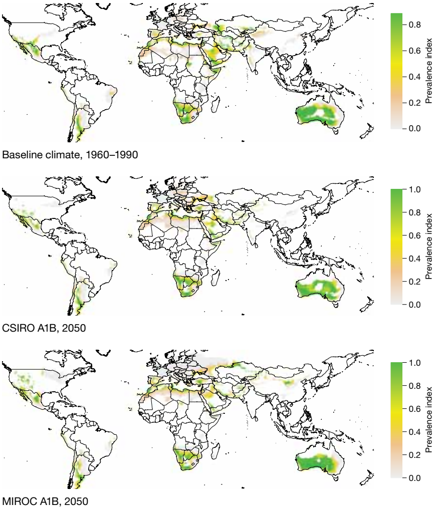
FIGURE C.10 Prevalence of wheat pest (Russian wheat aphid) under baseline climate, CSIRO A1B, and MIROC A1B scenarios
