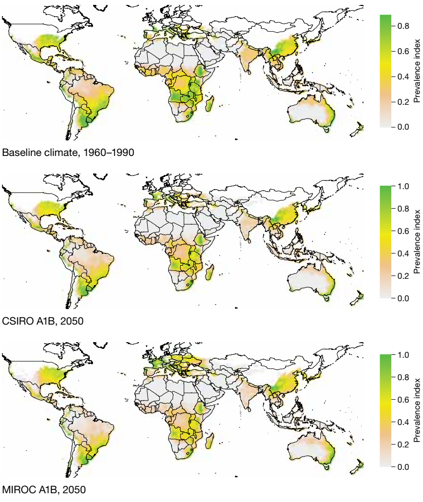
FIGURE C.5 Prevalence of maize weed (lambsquarters) under baseline climate, CSIRO A1B, and MIROC A1B scenarios
