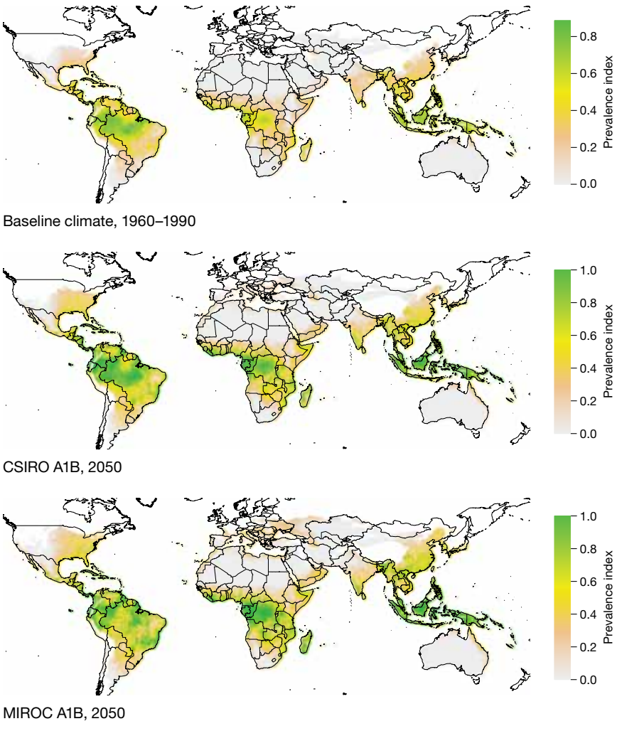
FIGURE C.7 Prevalence of rice disease (rice blast) under current baseline, CSIRO A1B, and MIROC A1B scenarios
