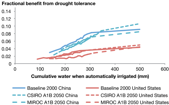
FIGURE A.6 Ex ante yield benefits of drought tolerance compared to the original variety under three different climate scenarios, winter wheat, China and the United States
