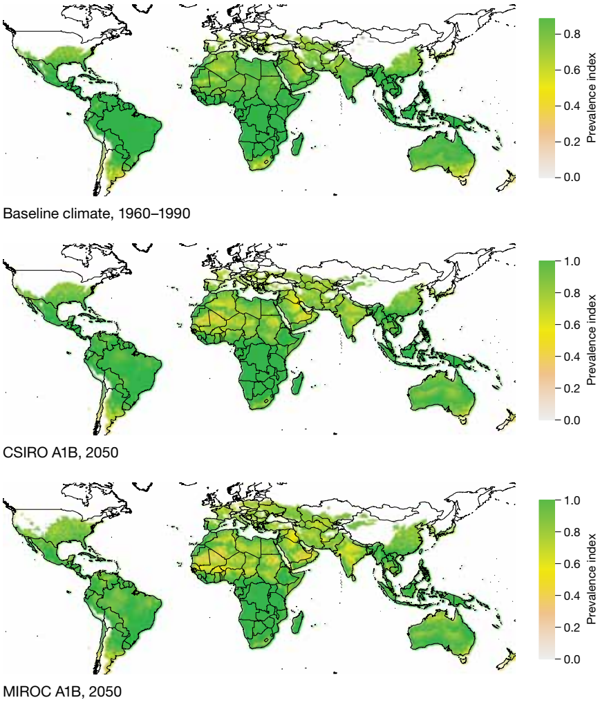
FIGURE C.3 Prevalence of maize pest (European corn borer) under baseline climate, CSIRO A1B, and MIROC A1B scenarios
