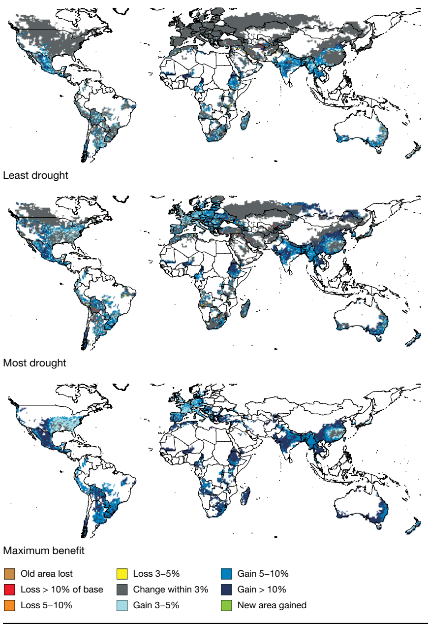
FIGURE A.4B Drought impact maps for winter wheat, CSIRO A1B scenario, 2050
