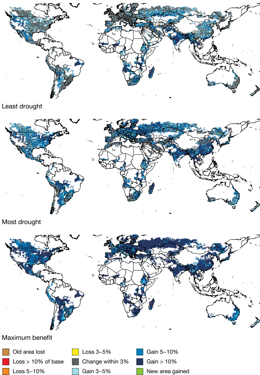
FIGURE A.3B Drought impact maps for spring wheat, CSIRO A1B scenario, 2050
