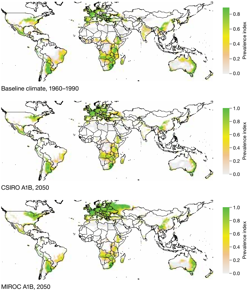
FIGURE C.11 Prevalence of wheat weed (wild oat) under baseline climate, CSIRO A1B, and MIROC A1B scenarios
