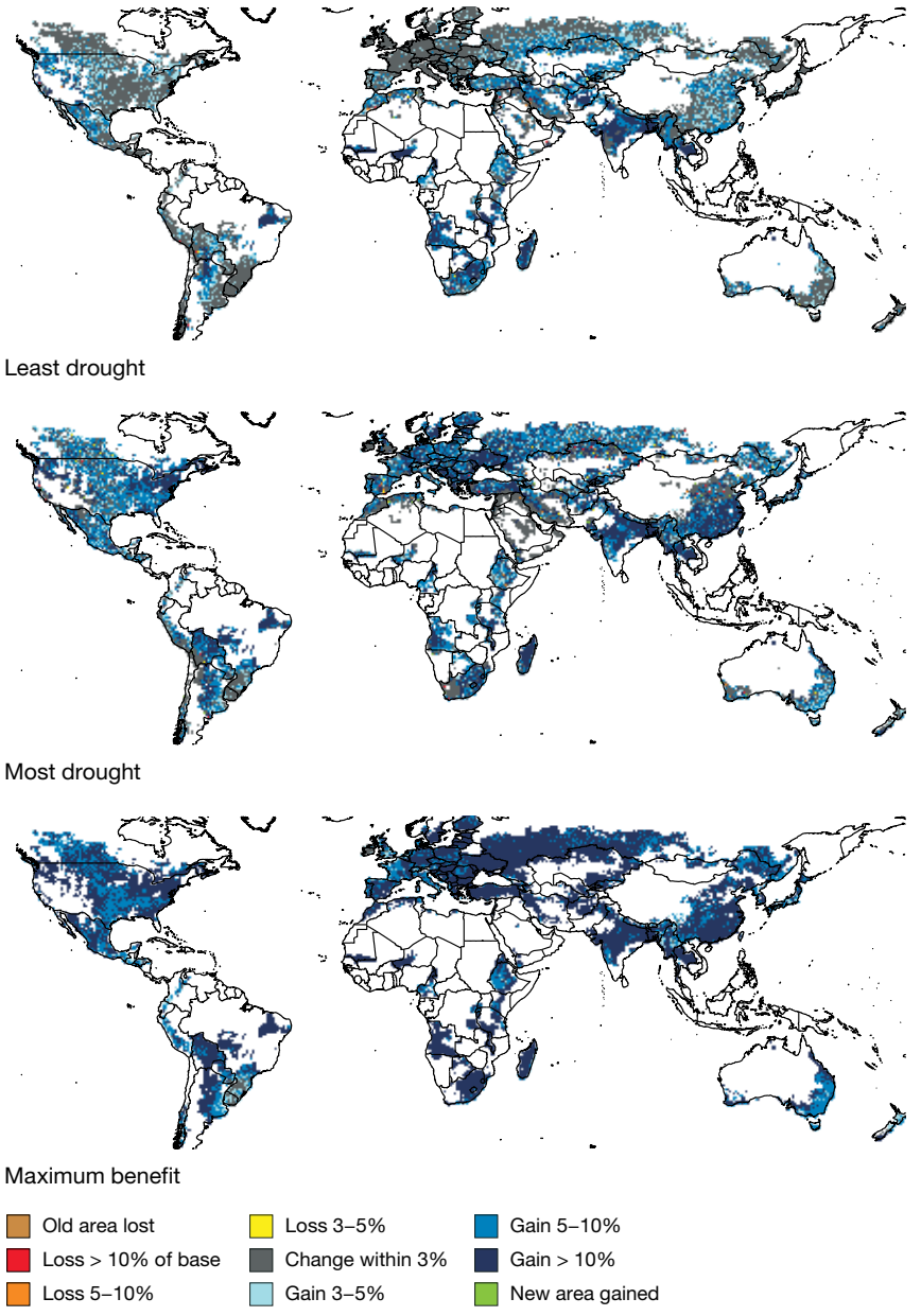
FIGURE A.3A Drought impact maps for spring wheat, baseline scenario, 2000
