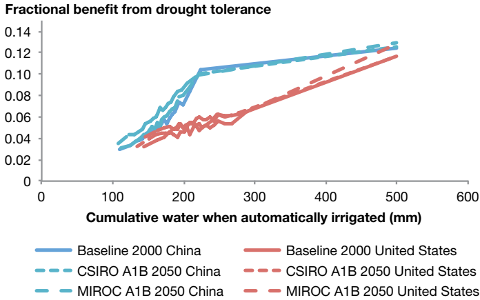
FIGURE A.5 Ex ante yield benefits of drought tolerance compared to the original variety under three different climate scenarios, spring wheat, China and the United States
